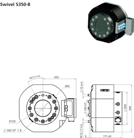
P0609 Swivel S350-8
