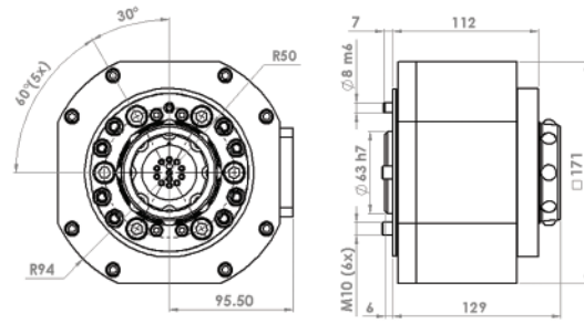
P0402 Tool attachment TA100-8, square
