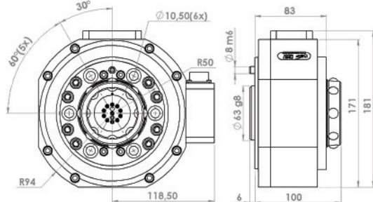
P0409 Tool attachment TA100-8E, round
