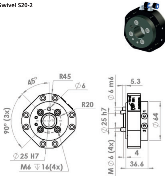
P0110A Swivel S20-2
