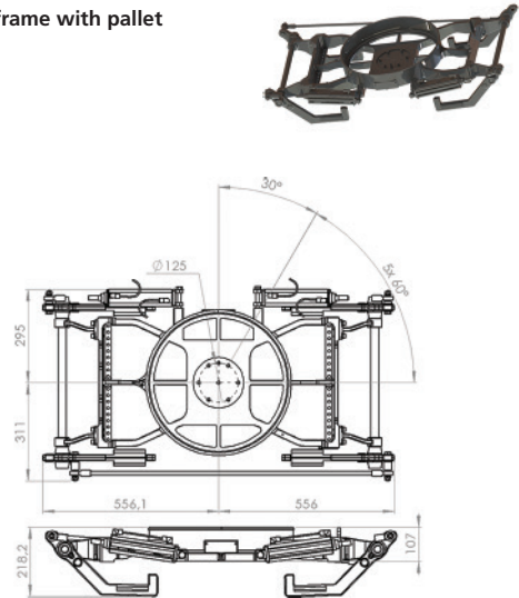
P9006 Adaptation kit for ABB IRB 66xx
