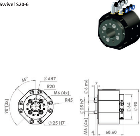
P0112A Swivel S20-6
